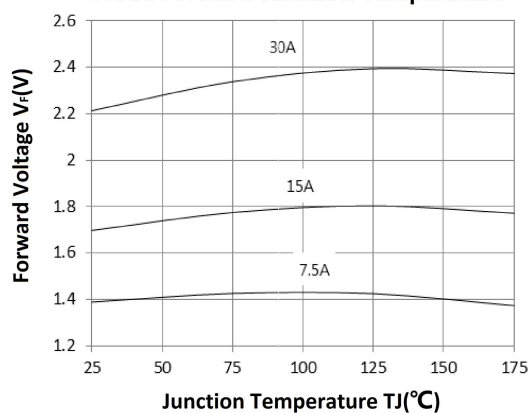
Diode Forward-Junction Temperature
