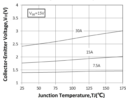
Typical Collector-Emitter Saturation Voltage-Junction Temperature
