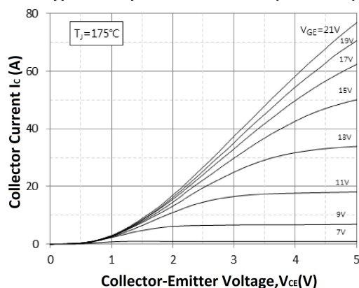
Typical Output Characteristics( T_J=175^\circ\text{C} )
